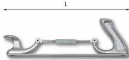
416 N Adjustable file holder - Screw adjustment for matching straight or curved contours - Adjustable for two lengths: 300 and 350 mm
